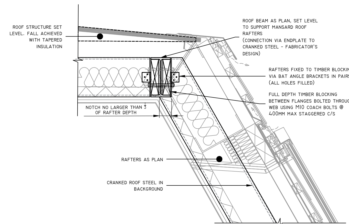
MANSARD ROOF / FLAT ROOF TRANSITION DETAIL ARCHITECT DETAIL REF: A817-T-2012A 1:10 @ A1 1:20 @ A3
