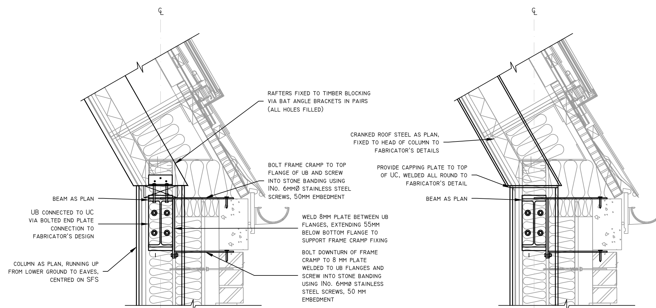
TOP OF WALL / EAVES DETAIL SHOWING RAFTER TO WALL PLATE AND CRANKED STEEL TO COLUMN ARCHITECT DETAIL REF: A817-T-2011B 1:10 @ A1 1:20 @ A3
