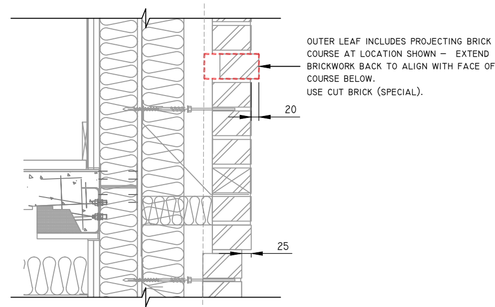
PROJECTING BRICK COURSE DETAIL ARCHITECT DETAIL REF: A817-T-2010A 1:10 @ A1 1:20 @ A3
