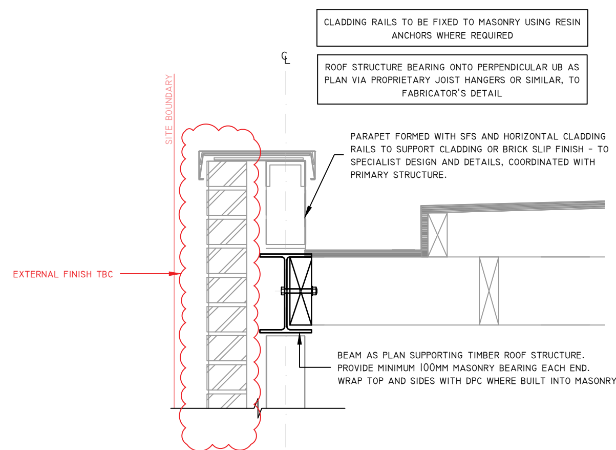
PLANT ROOF PARAPET DETAIL ARCHITECT DETAIL REF: A817-T-2020B 1:10 @ A1 1:20 @ A3
