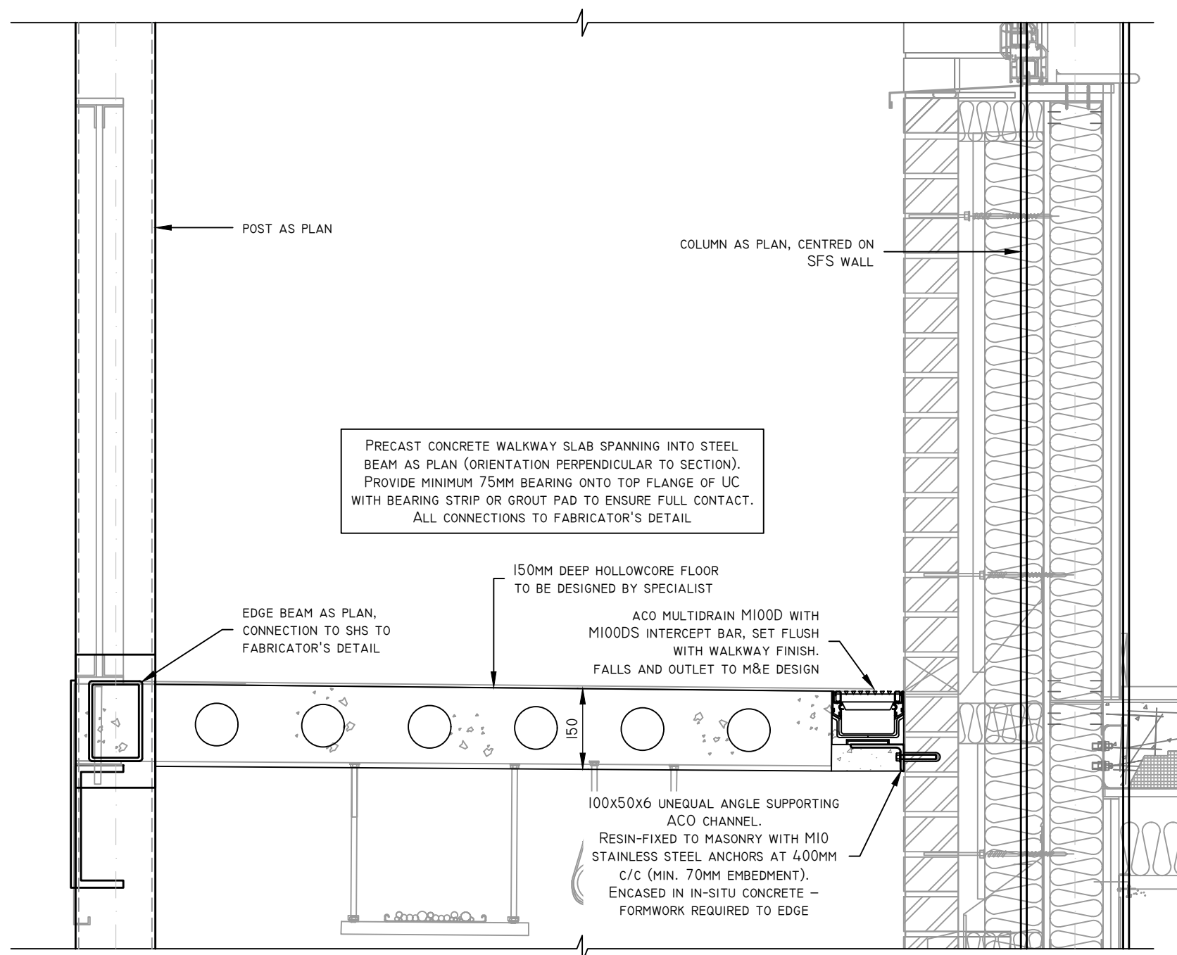
WALKWAY / ROOF INTERFACE DETAIL - COLUMN OR STUB CONNECTION OPTION ARCHITECT DETAIL REF: A817-T-2014A 1:10 @ A1 1:20 @ A3
