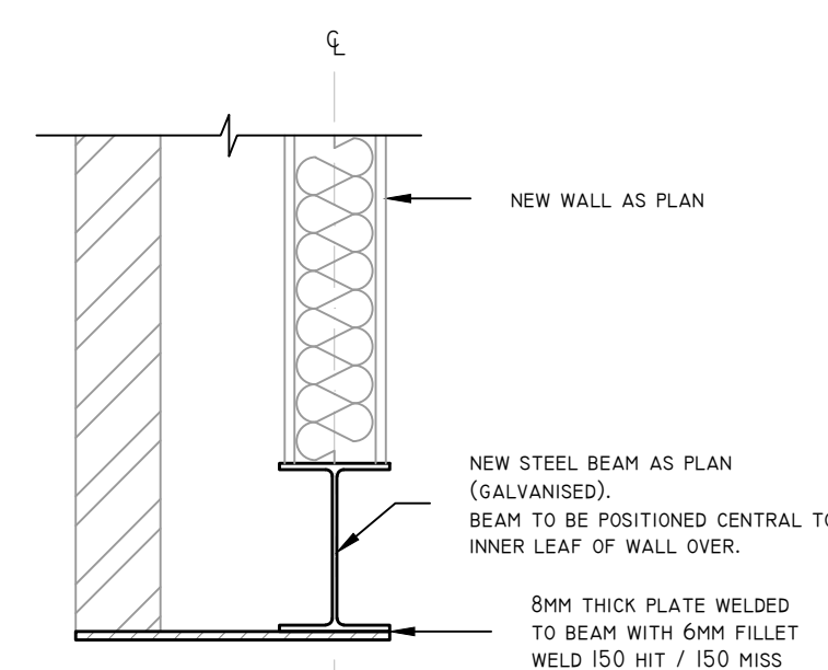
MASONRY SUPPORT DETAIL 1:10 @ A1 1:20 @ A3
