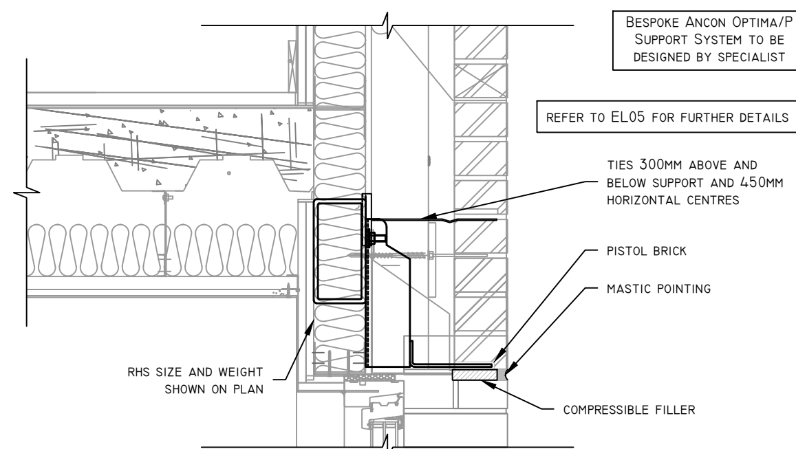
MASONRY SUPPORT ANGLE DETAIL ARCHITECT DETAIL REF: A817-T-2004A 1:10 @ A1 1:20 @ A3
